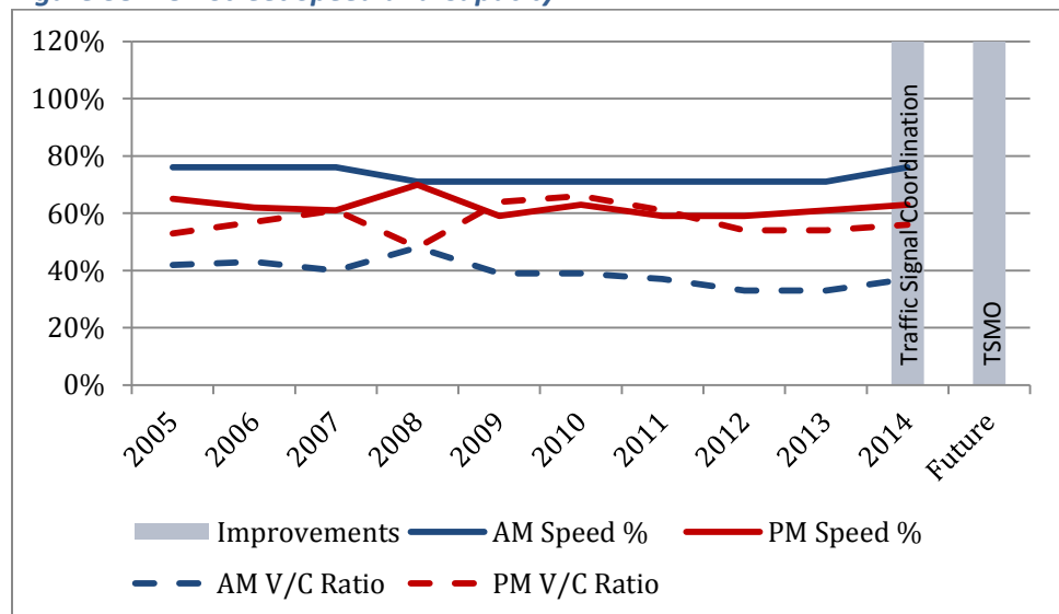
Figure 38: 78 th Street Speed and Capacity
