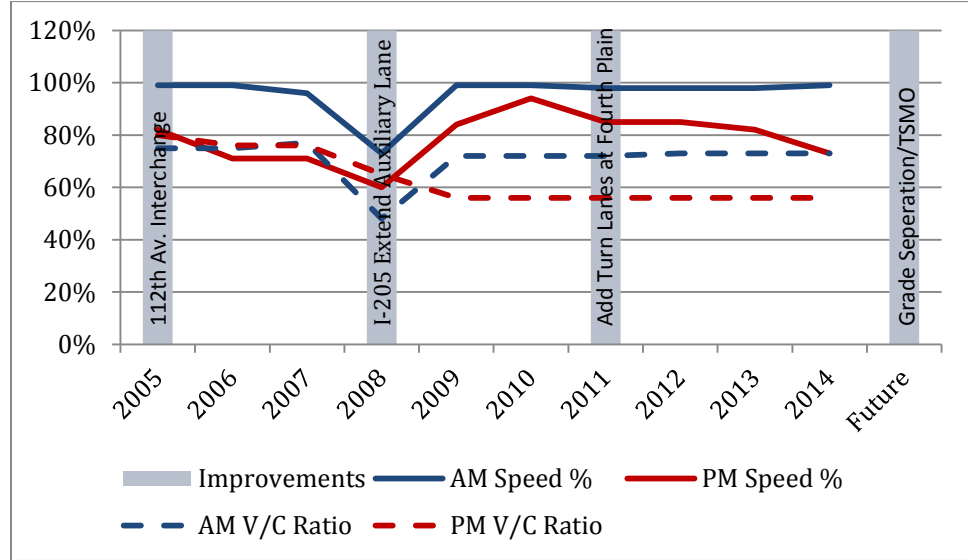
Figure 35: SR-500 Central Speed and Capacity
