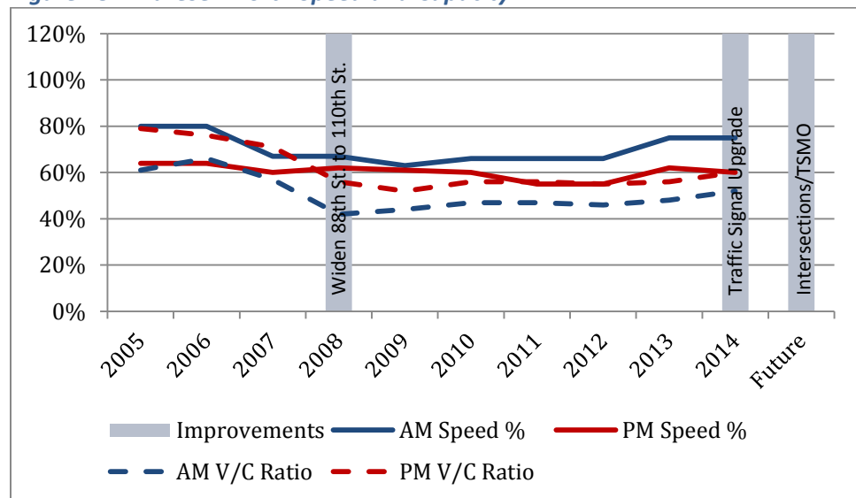
Figure 18: Andresen North Speed and Capacity
