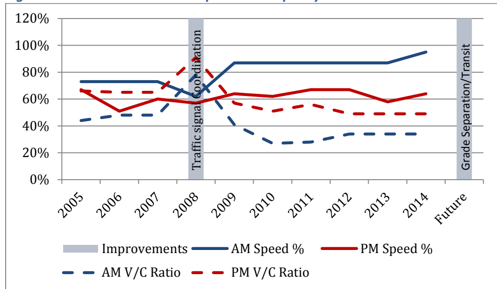
Figure 36: Fourth Plain Central Speed and Capacity
