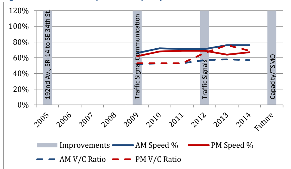
Figure 25: 192 nd Avenue Speed and Capacity
