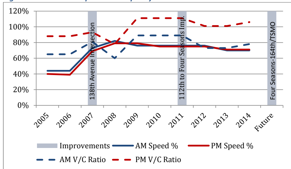
Figure 42: 18 th Street Speed and Capacity
