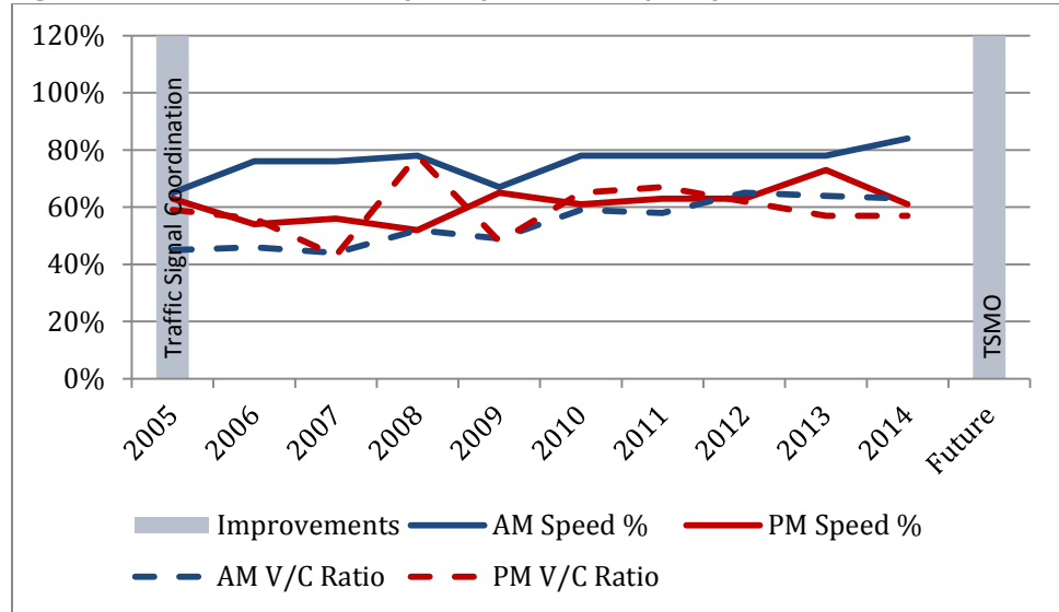
Figure 29: Fourth Plain west of I-5 Speed and Capacity
