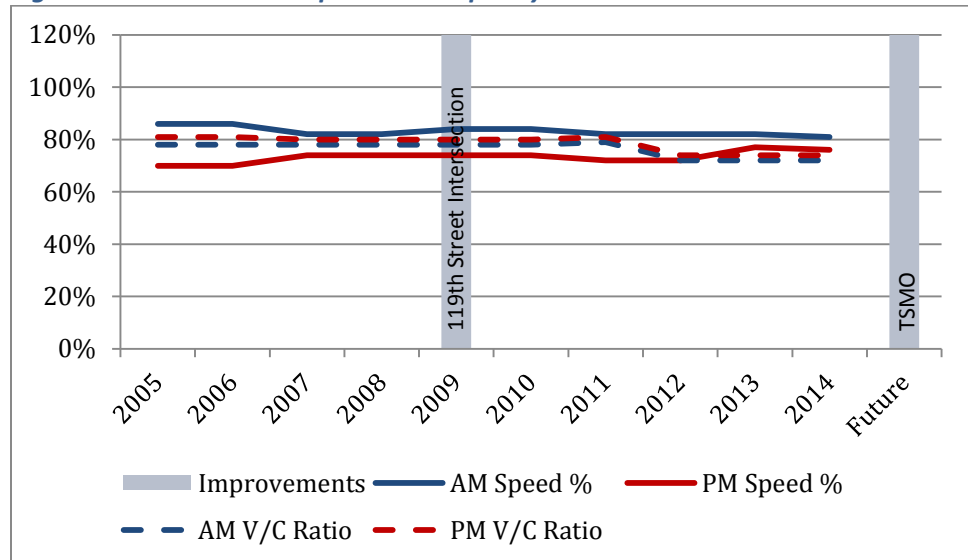
Figure 20: SR-503 North Speed and Capacity
