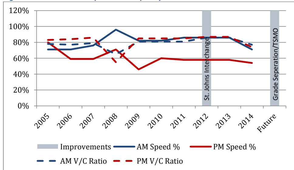
Figure 34: SR-500 West Speed and Capacity
