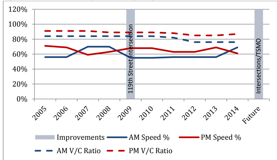
Figure 21: SR-503 South Speed and Capacity
