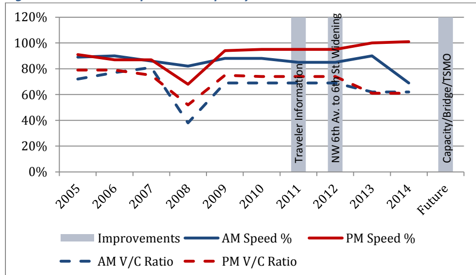
Figure 28: SR-14 East Speed and Capacity
