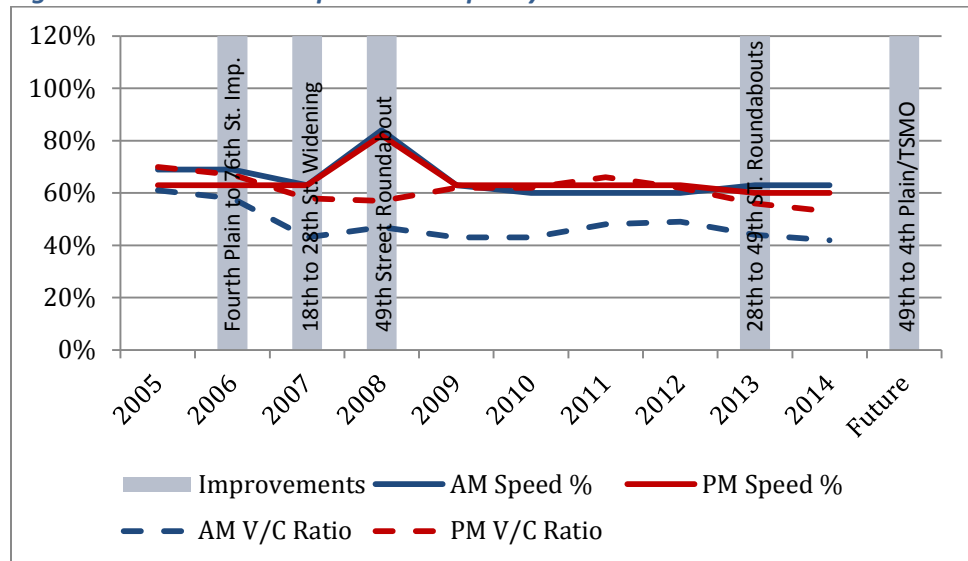
Figure 22: 137 th Avenue Speed and Capacity
