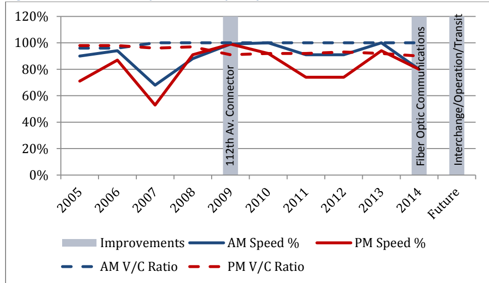
Figure 15: I-205 South Speed and Capacity
