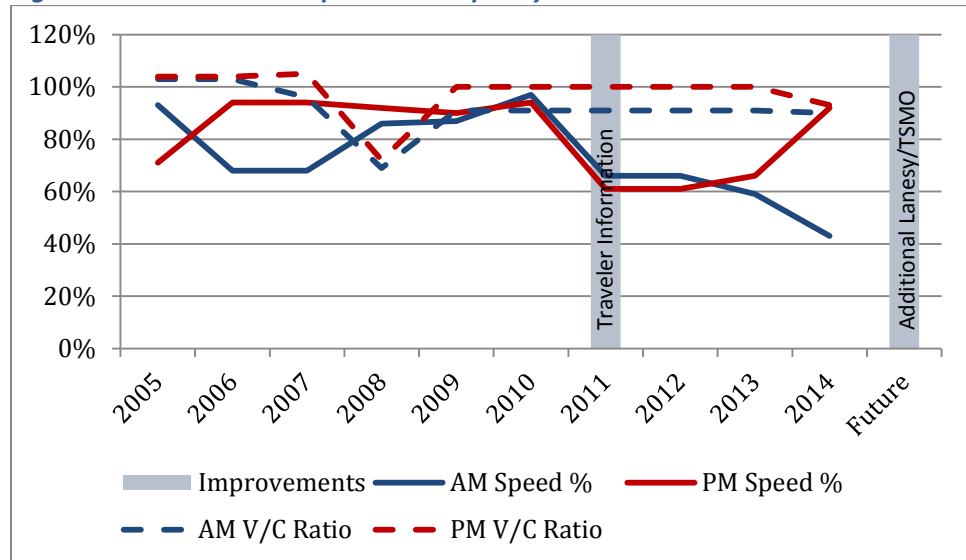
Figure 27: SR-14 Central Speed and Capacity
