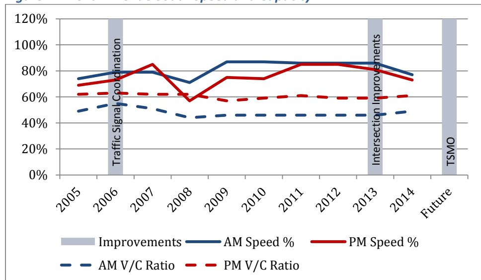
Figure 24: 164th Avenue South Speed and Capacity
