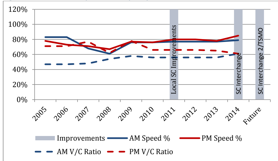
Figure 43: 134 th Street Speed and Capacity
