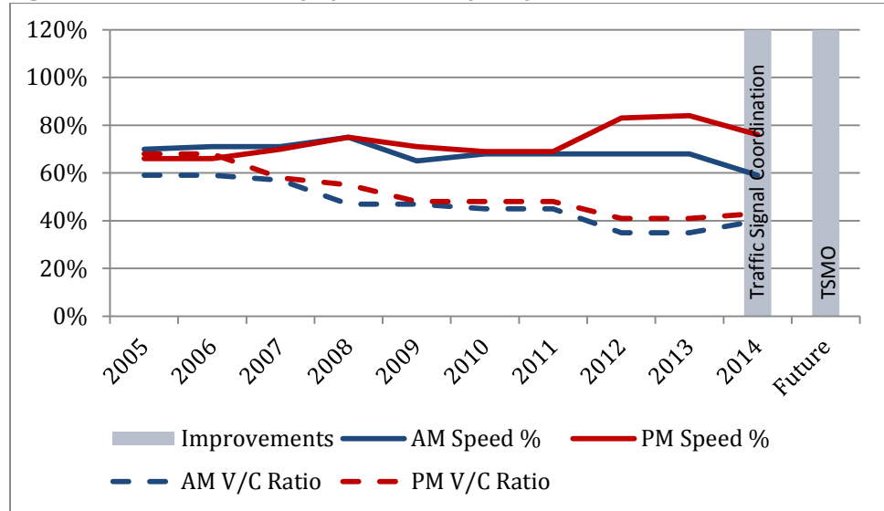
Figure 39: Padden Parkway Speed and Capacity
