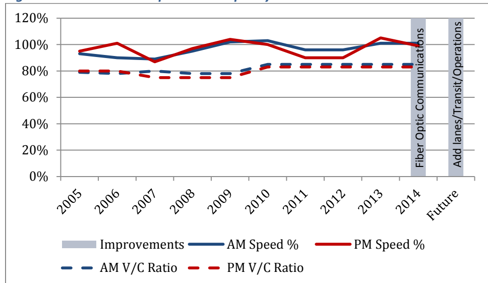
Figure 14: I-205 Central Speed and Capacity
