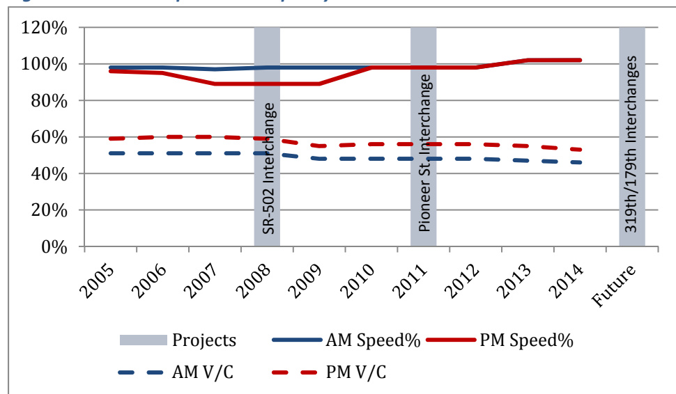
Figure 8: I-5 North Speed and Capacity
