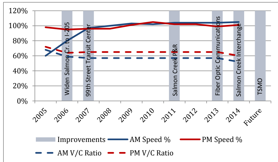
Figure 9: I-5 Central Speed and Capacity
