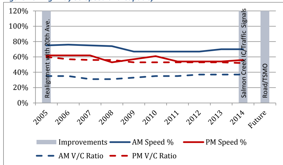
Figure 10: Highway 99 Speed and Capacity
