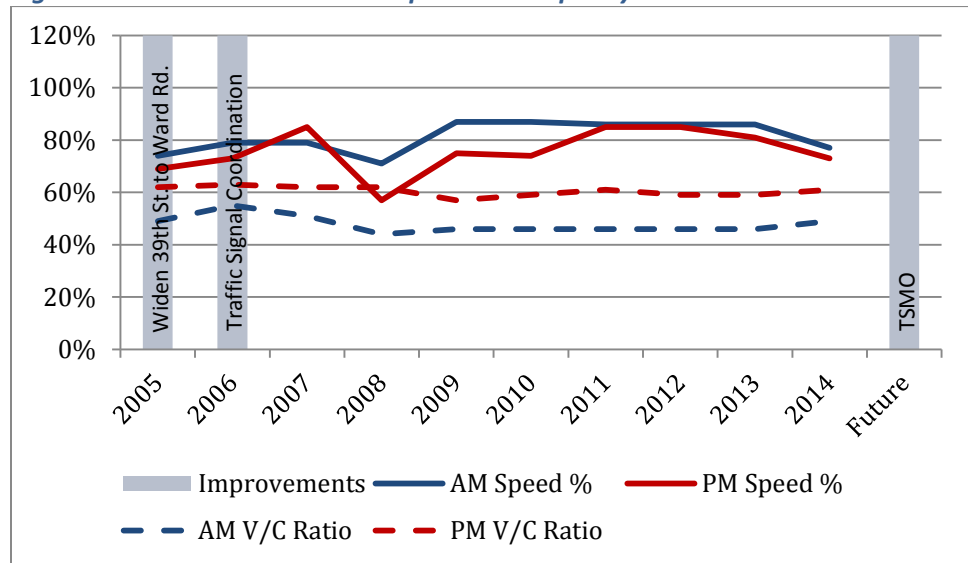
Figure 23: 162nd Avenue North Speed and Capacity
