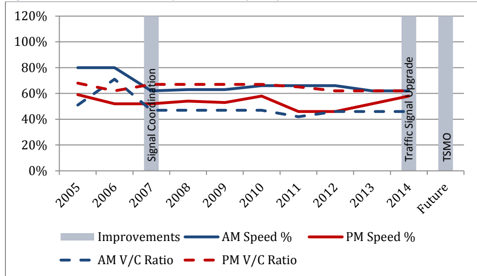
Figure 19: Andresen South Speed and Capacity
