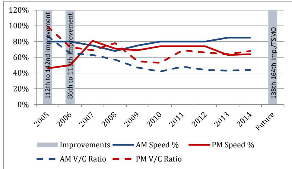
Figure 41: Burton Road Speed and Capacity
