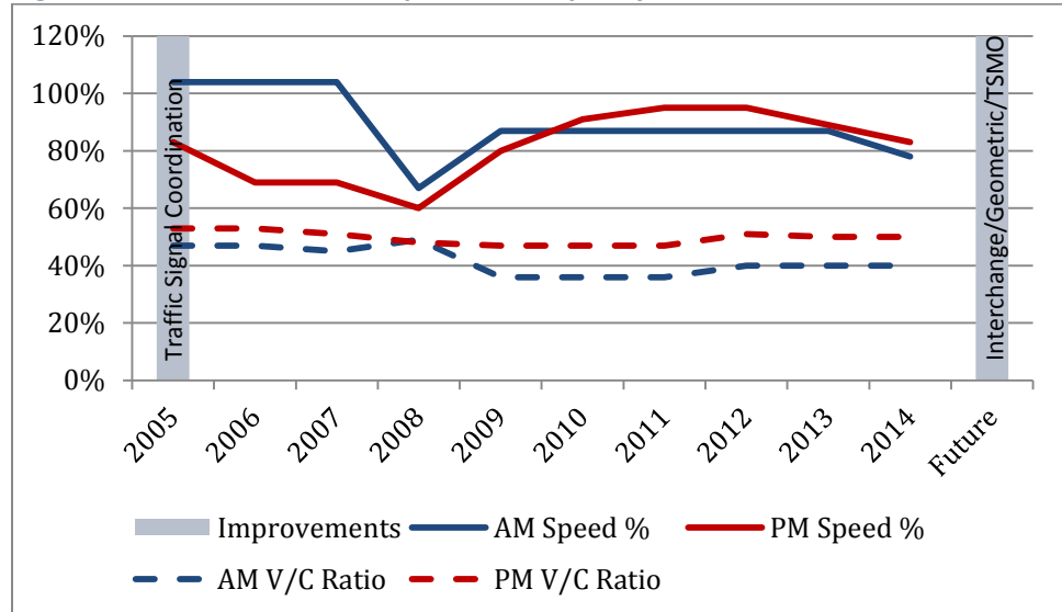
Figure 30: SR-501/Mill Plain Speed and Capacity
