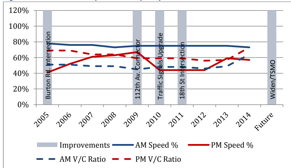
Figure 16: 112 th Avenue Speed and Capacity
