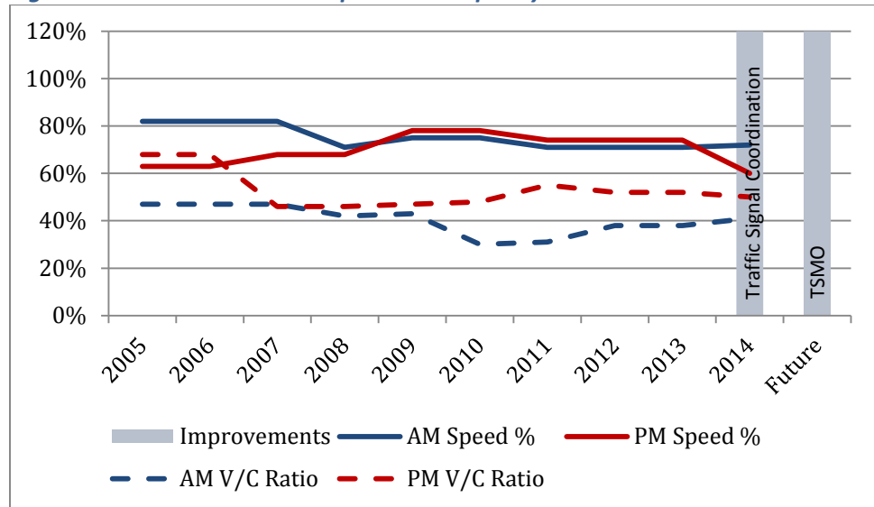
Figure 11: Hazel Dell Avenue Speed and Capacity
