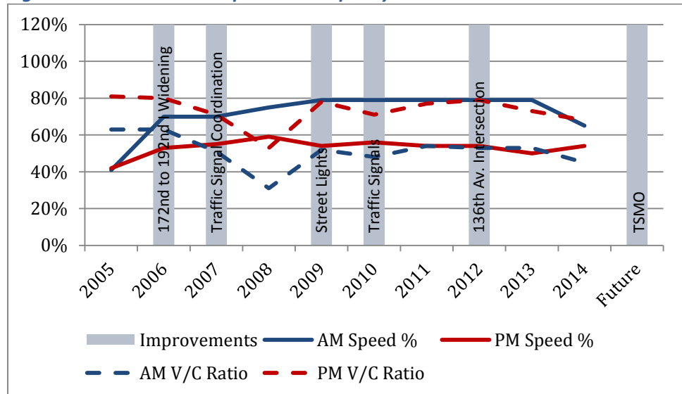
Figure 32: Mill Plain East Speed and Capacity
