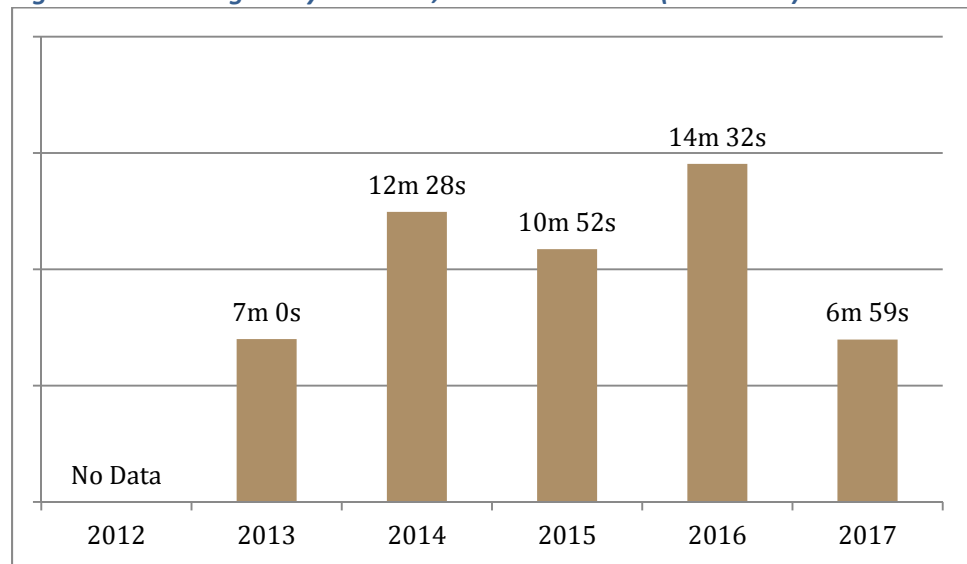
Figure 51: Morning Delay on SR-14, 192 nd AV to I-205 (4.16 miles)
