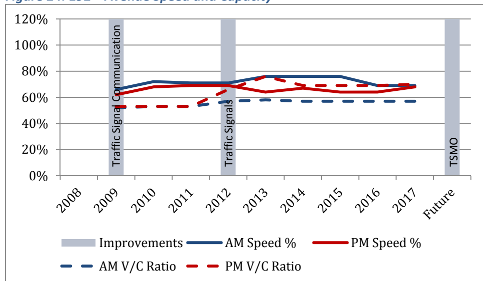
Figure 24: 192 nd Avenue Speed and Capacity
